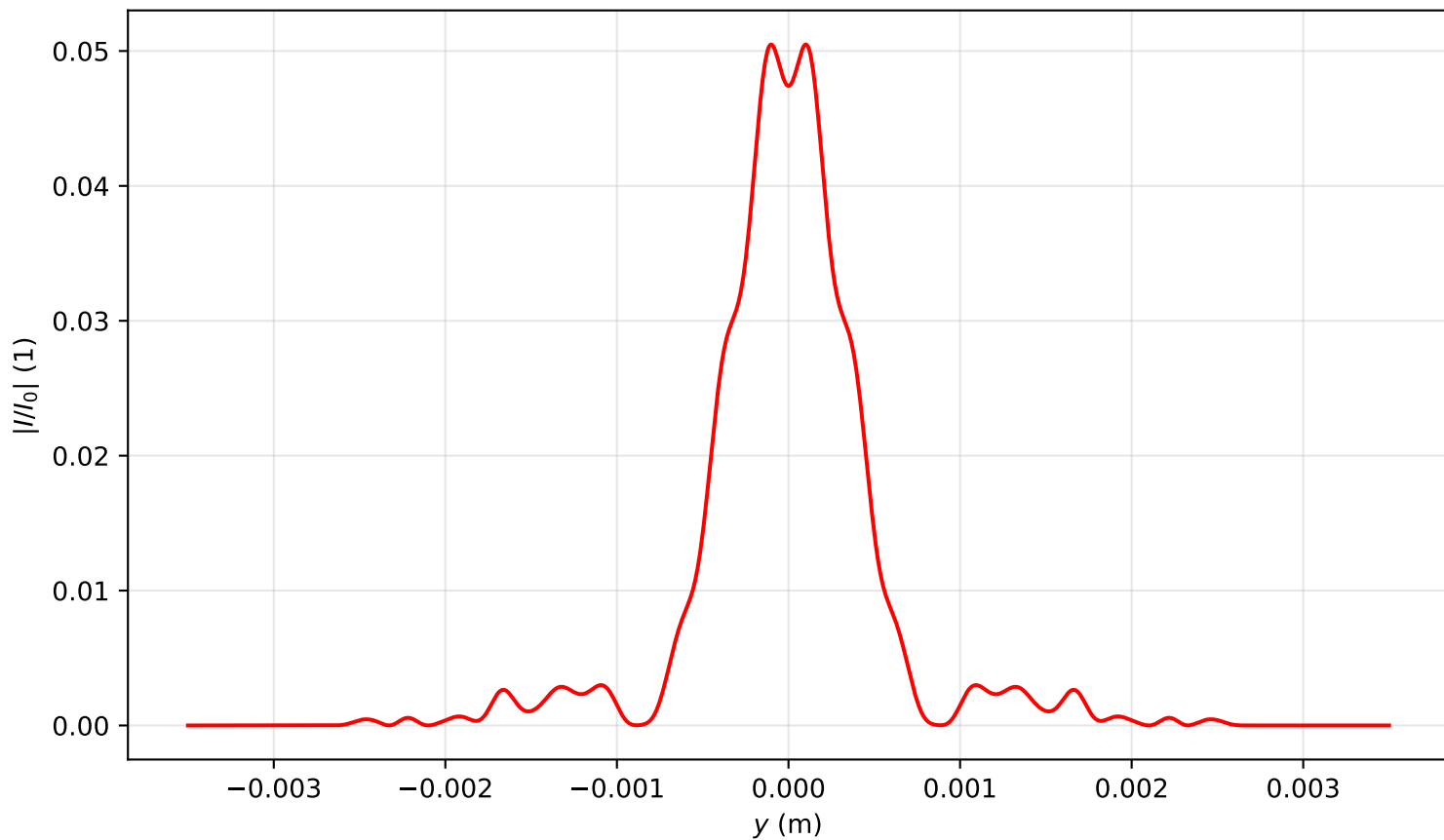
Intensity profile I(x=0, y, z=1.911)/I_0 , P_{in}=19.0P_{cr} , artificial time
