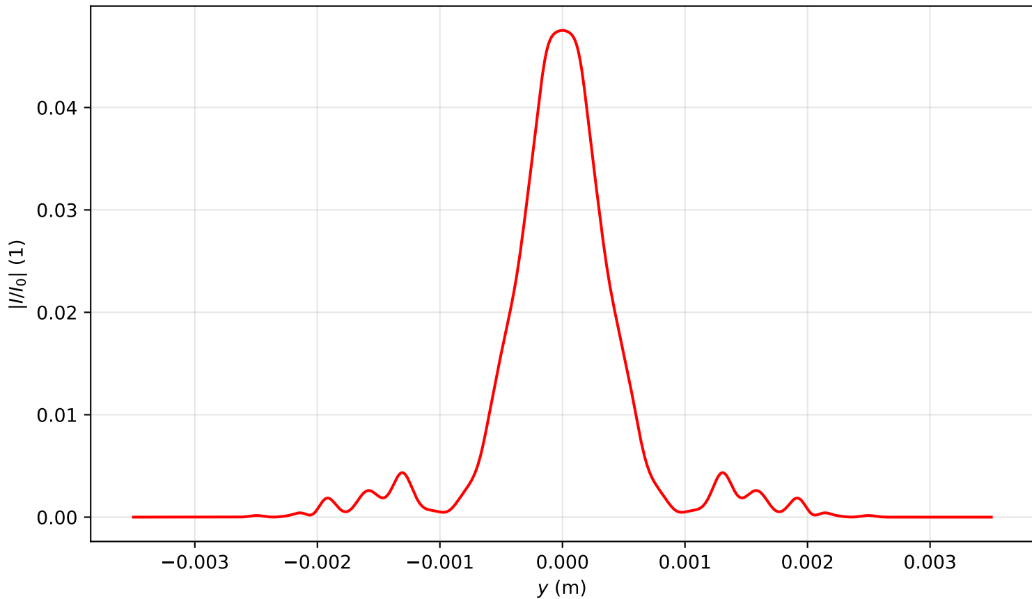
Intensity profile I(x=0, y, z=2.070)/I_0 , P_{in}=19.0\text{Pcr} , artificial time
