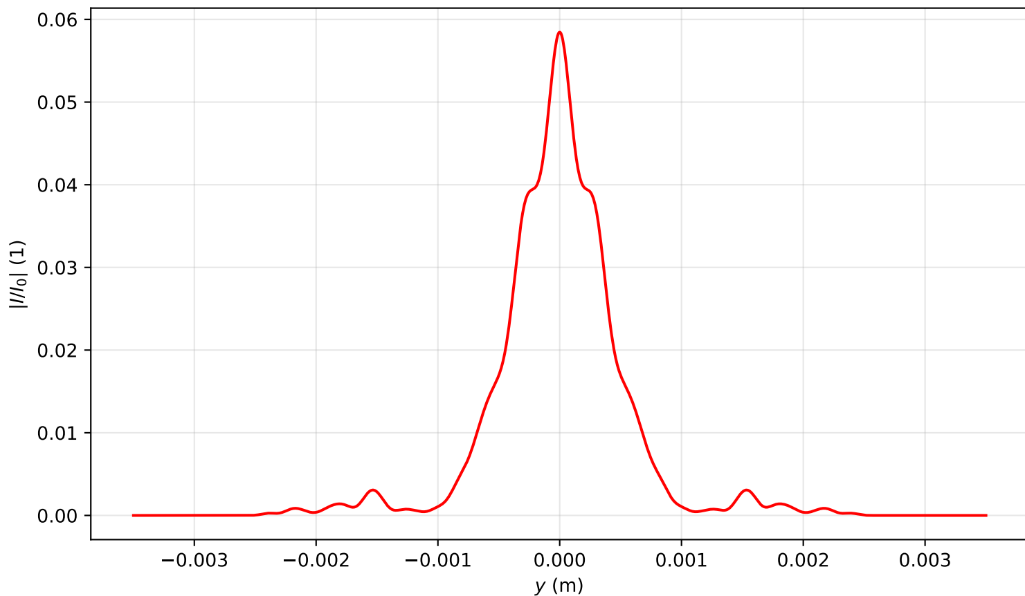
Intensity profile I(x=0, y, z=2.229)/I_0 , P_{in}=19.0\text{Pcr} , artificial time
