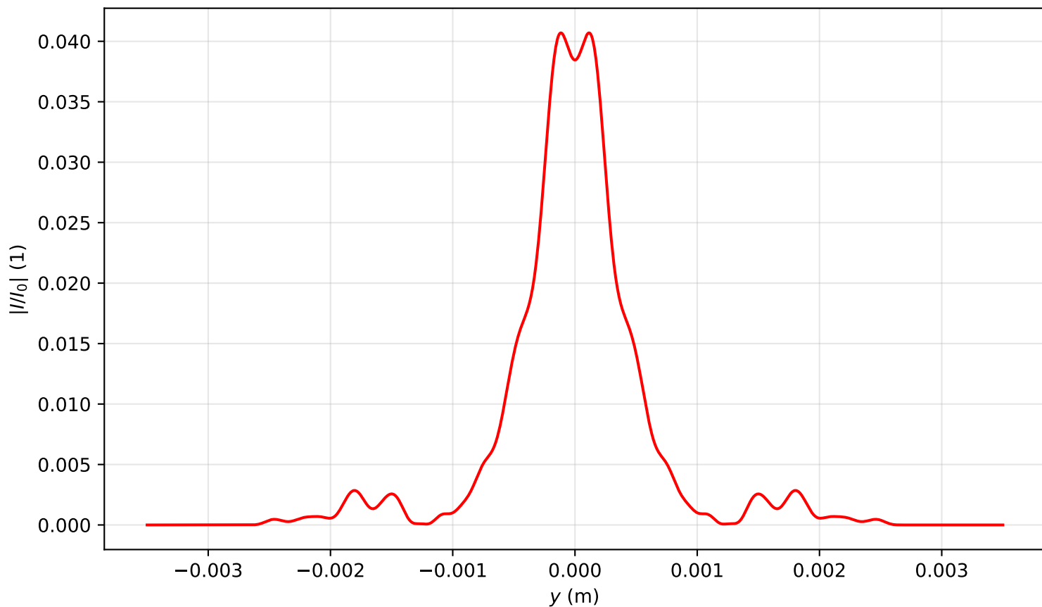
Intensity profile I(x=0, y, z=2.388)/I_0 , P_{in}=19.0P_{cr} , artificial time
