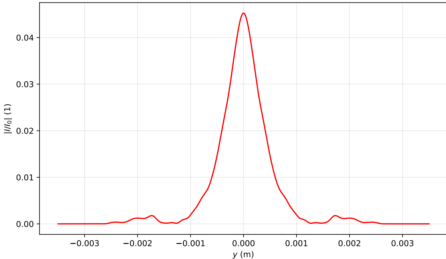
Intensity profile I(x = 0, y, z = 2.548)/I_0 , P_{in}=19.0\text{Pcr} , artificial time
