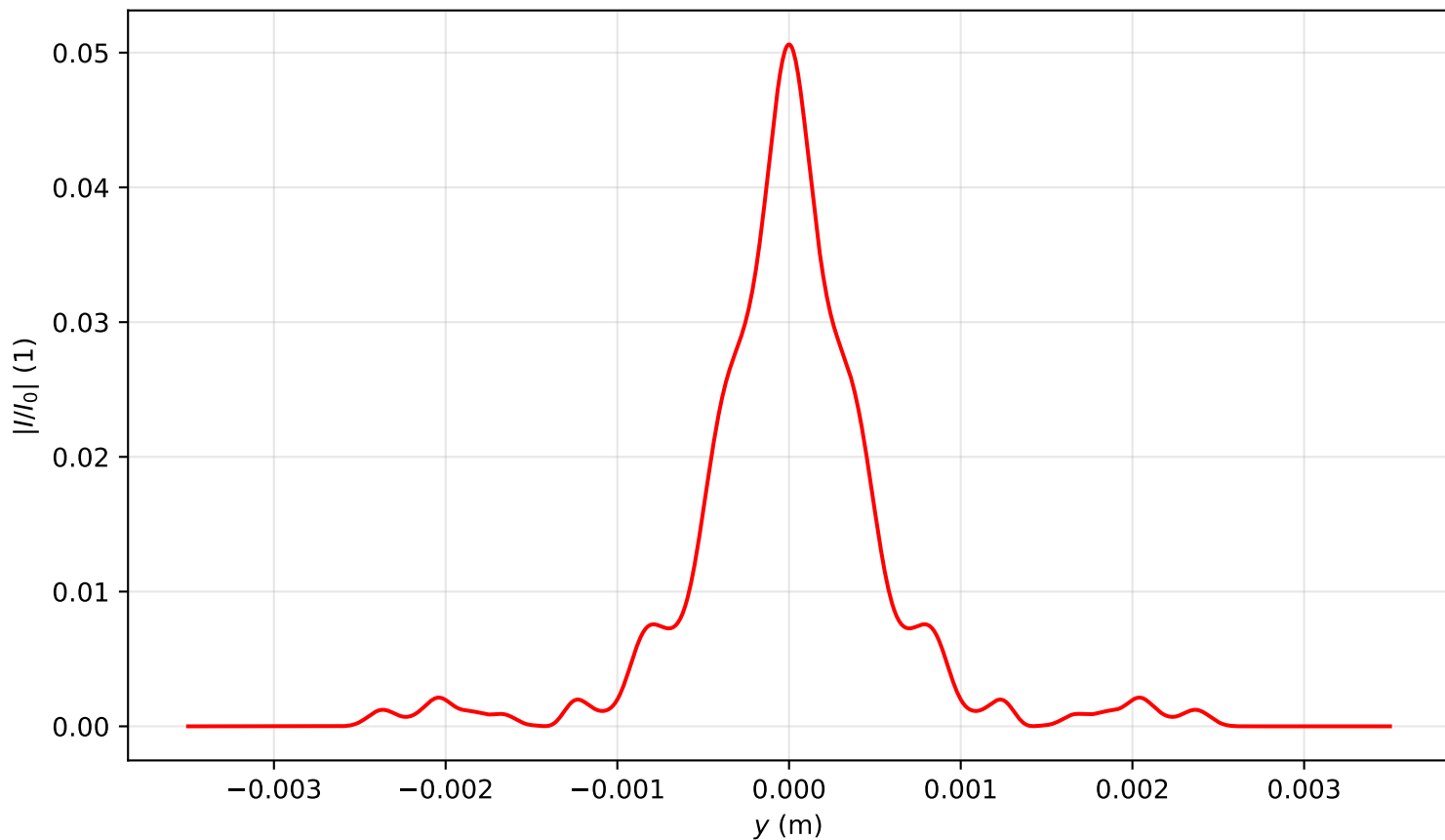
Intensity profile I(x = 0, y, z = 2.707)/I_0 , P_{in}=19.0P_{cr} , artificial time
