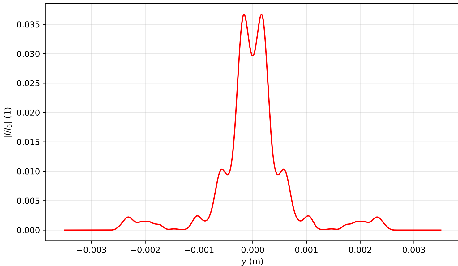
Intensity profile I(x=0, y, z=2.866)/I_0 , P_{in}=19.0\text{Pcr} , artificial time
