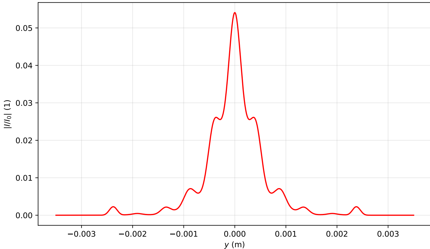
Intensity profile I(x = 0, y, z = 3.184)/I_0 , P_{in}=19.0\text{Pcr} , artificial time
