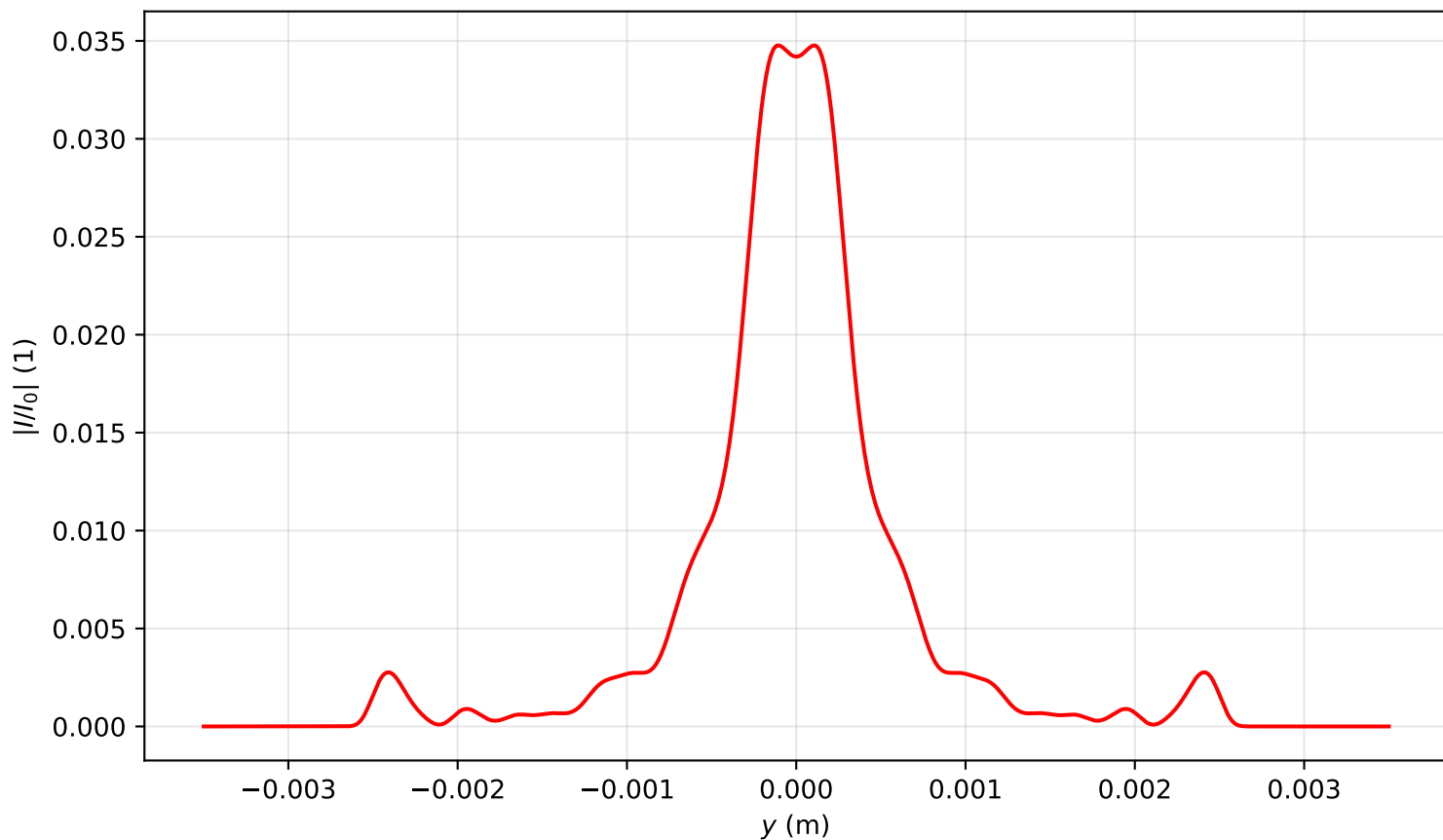
Intensity profile I(x=0, y, z=3.344)/I_0 , P_{in}=19.0\text{Pcr} , artificial time
