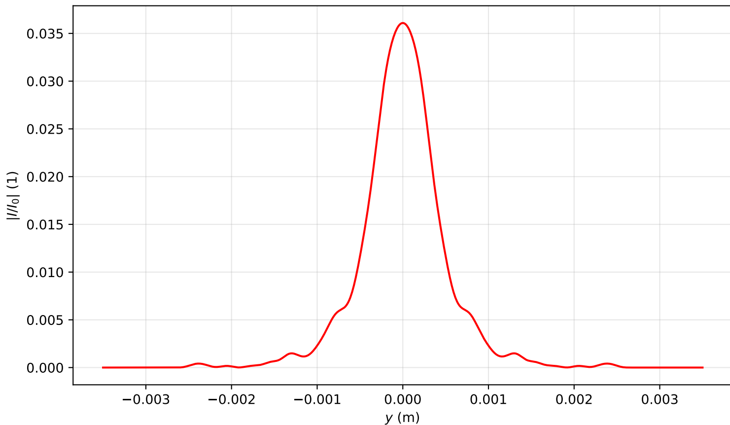
Intensity profile I(x=0, y, z=3.662)/I_0 , P_{in}=19.0\text{Pcr} , artificial time
