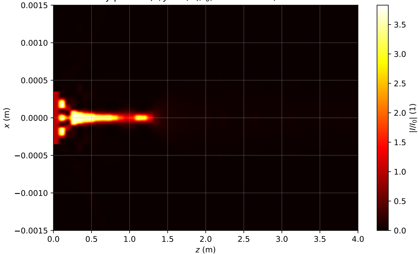
Intensity profile I(x, y = 0, z)/I_0 , P_{in}=19.0\text{Pcr} , artificial time
