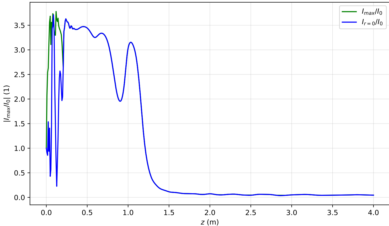
I_{\max}(x = 0, y = 0, z)/I_0 , \text{Pin}=20.0\text{Pcr} , artificial time
