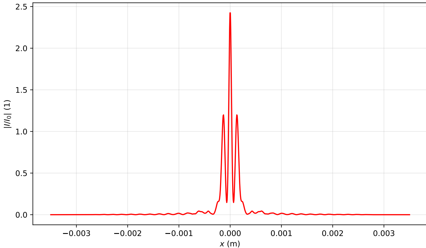
Intensity profile I(x, y = 0, z = 0.159)/I_0 , P_{in}=20.0P_{cr} , artificial time
