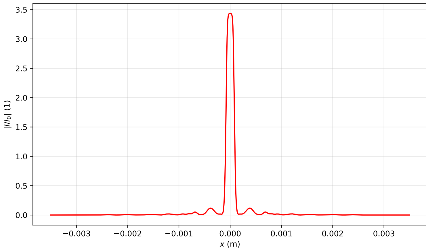
Intensity profile I(x, y = 0, z = 0.318)/I_0 , P_{in}=20.0P_{cr} , artificial time
