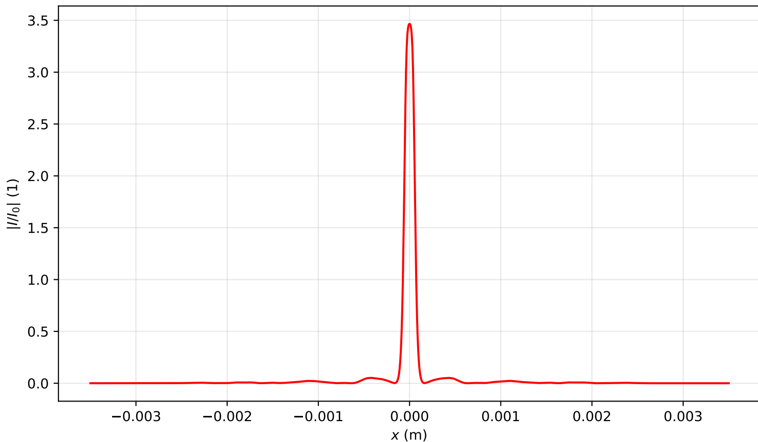
Intensity profile I(x, y = 0, z = 0.478)/I_0 , P_{in}=20.0P_{cr} , artificial time
