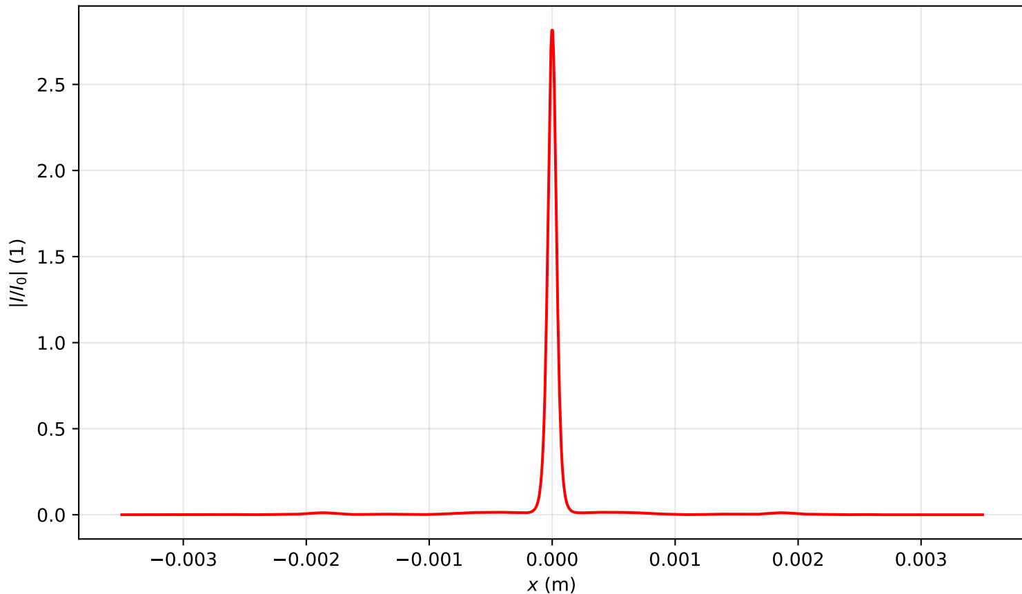
Intensity profile I(x, y = 0, z = 0.796)/I_0 , P_{in}=20.0P_{cr} , artificial time
