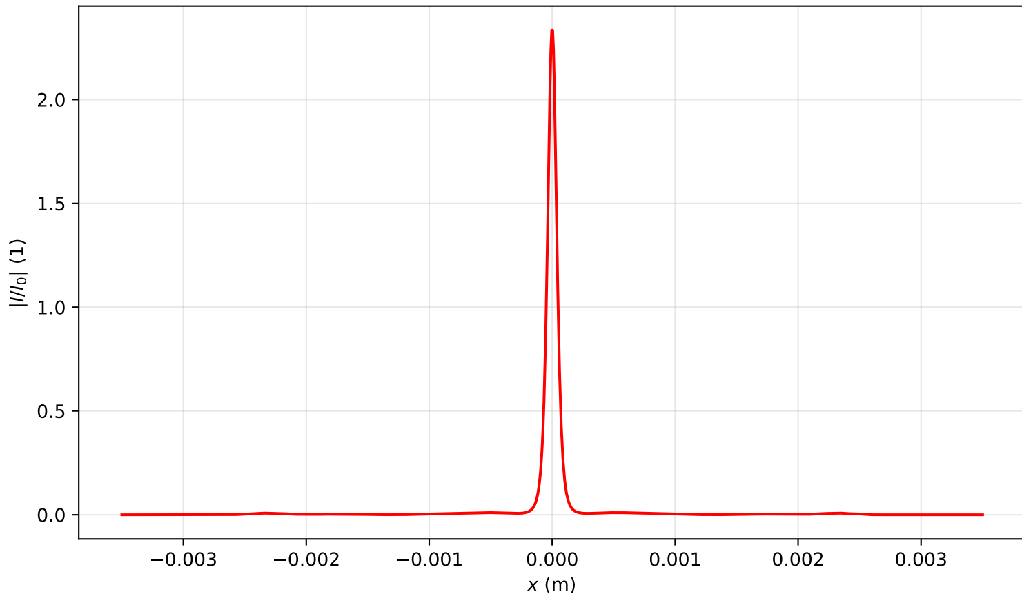
Intensity profile I(x, y = 0, z = 0.955)/I_0 , P_{in}=20.0P_{cr} , artificial time
