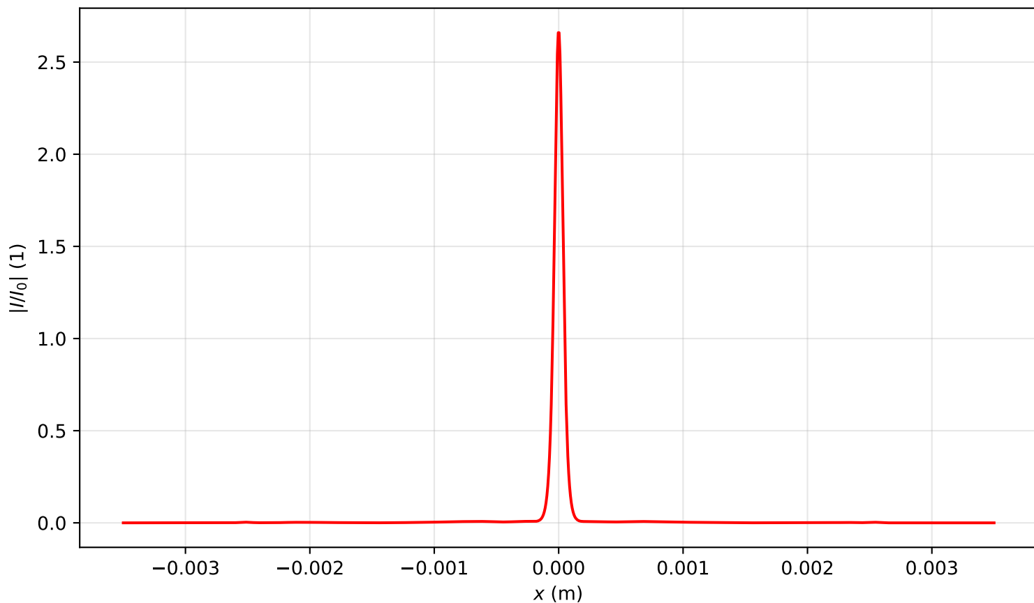
Intensity profile I(x, y = 0, z = 1.115)/I_0 , P_{in}=20.0P_{cr} , artificial time
