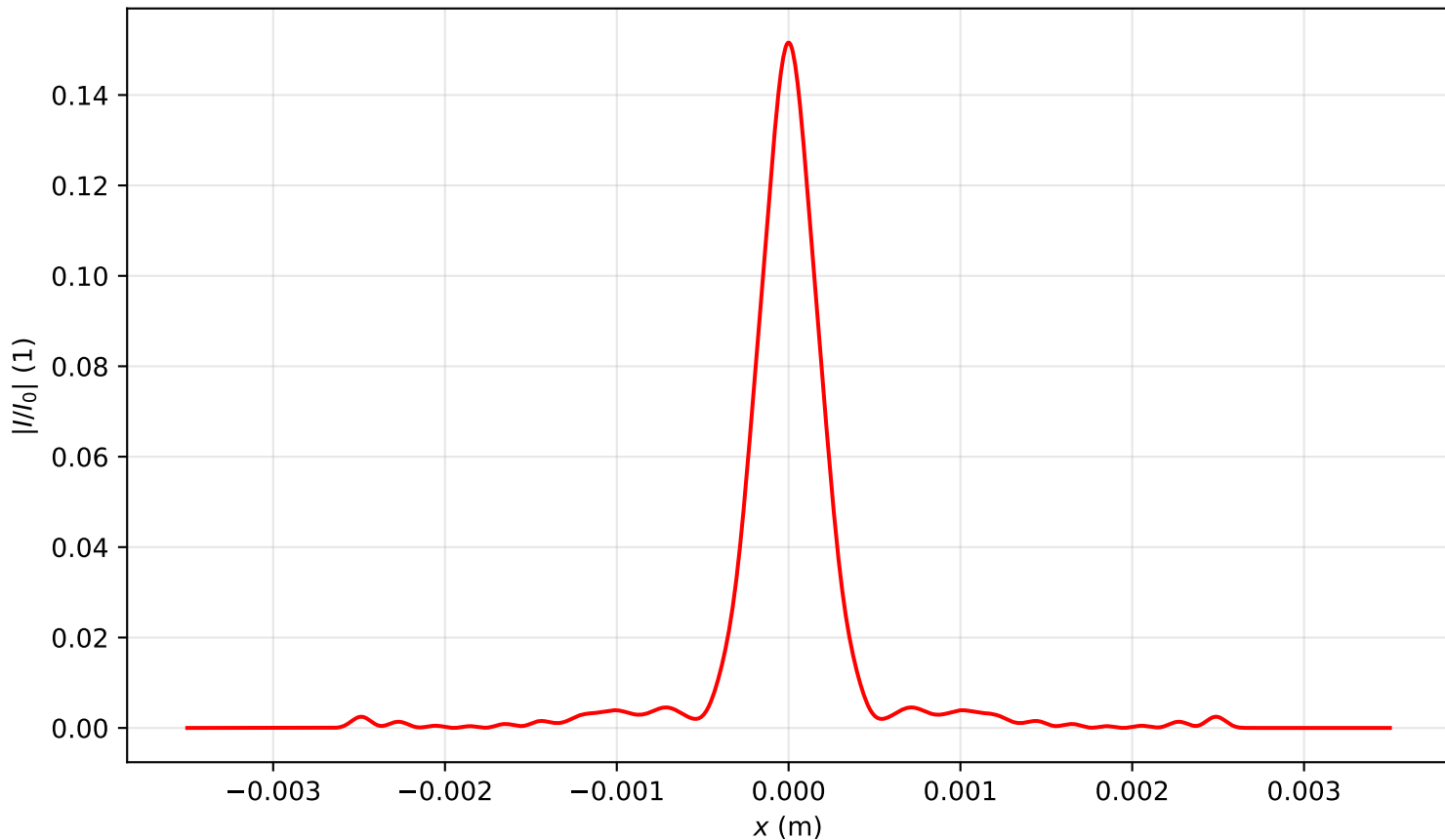
Intensity profile I(x, y = 0, z = 1.433)/I_0 , P_{in}=20.0\text{Pcr} , artificial time
