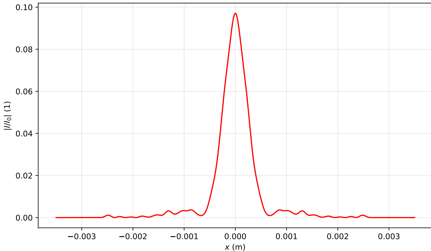
Intensity profile I(x, y = 0, z = 1.592)/I_0 , P_{in}=20.0P_{cr} , artificial time
