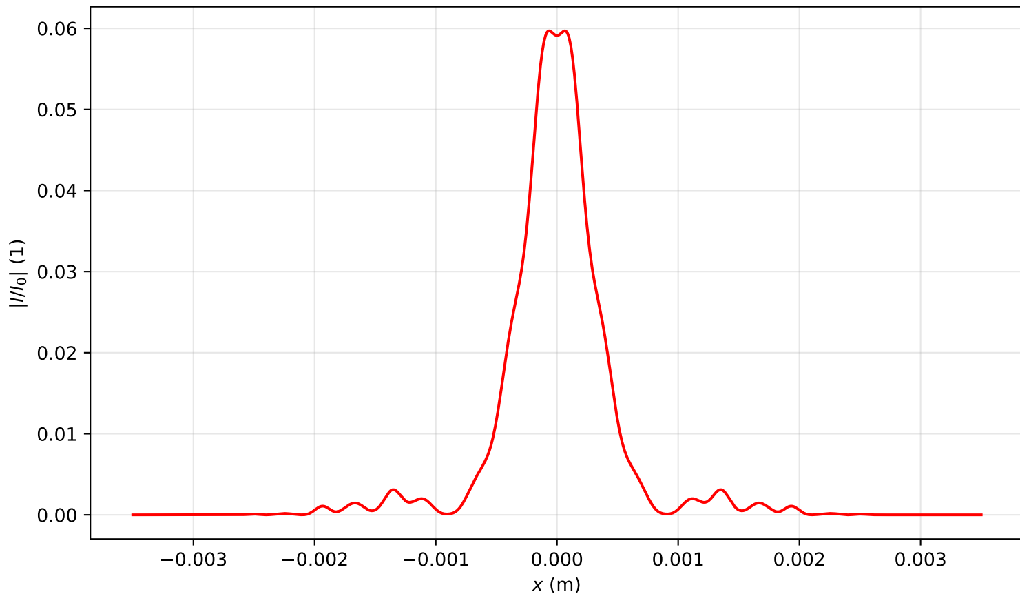
Intensity profile I(x, y = 0, z = 1.911)/I_0 , P_{in}=20.0\text{Pcr} , artificial time
