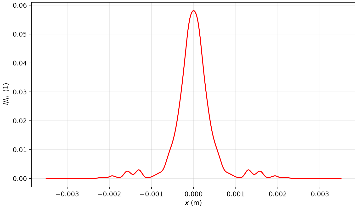
Intensity profile I(x, y = 0, z = 2.070)/I_0 , P_{in}=20.0P_{cr} , artificial time
