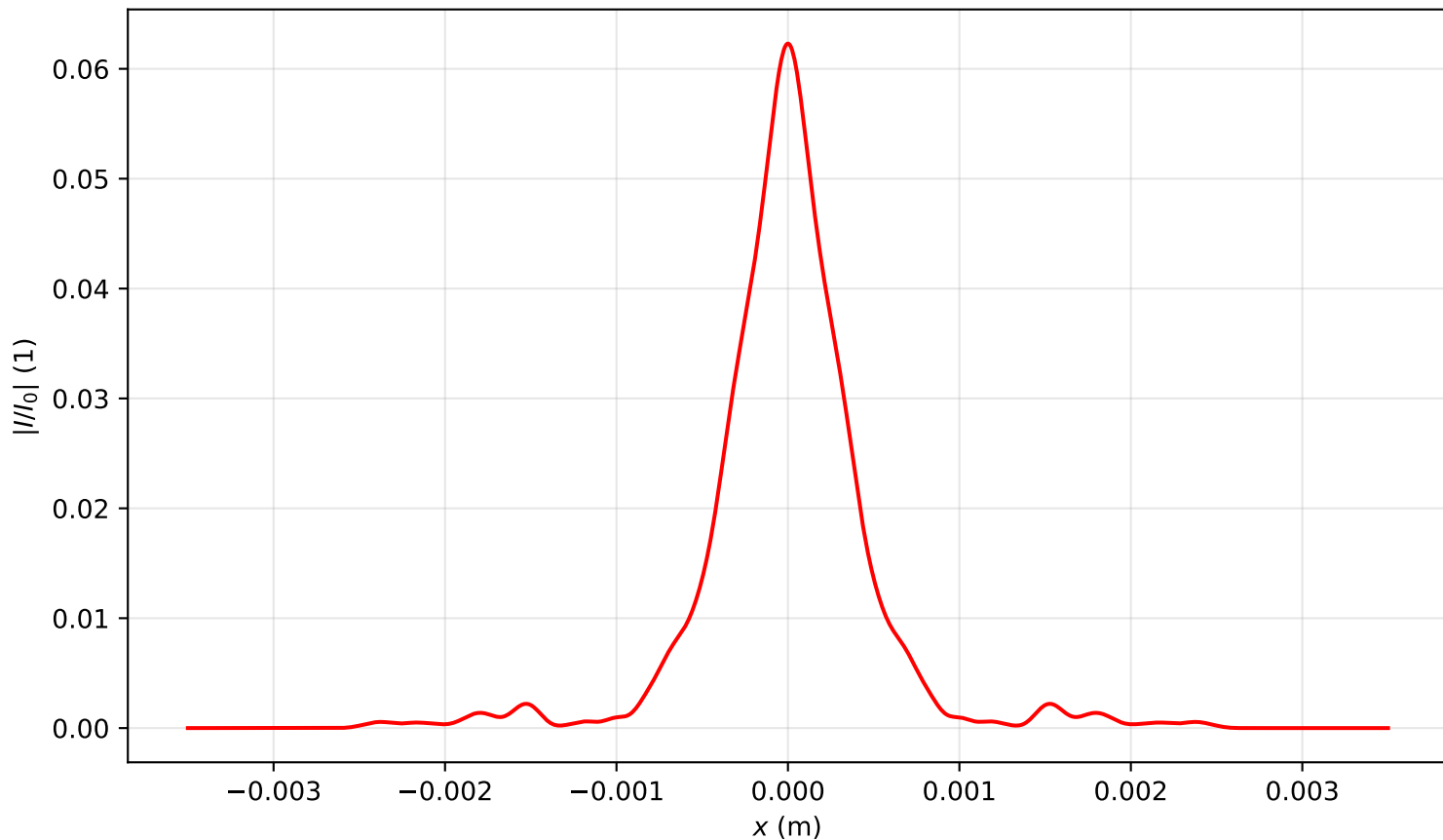
Intensity profile I(x, y = 0, z = 2.229)/I_0 , P_{in}=20.0P_{cr} , artificial time
