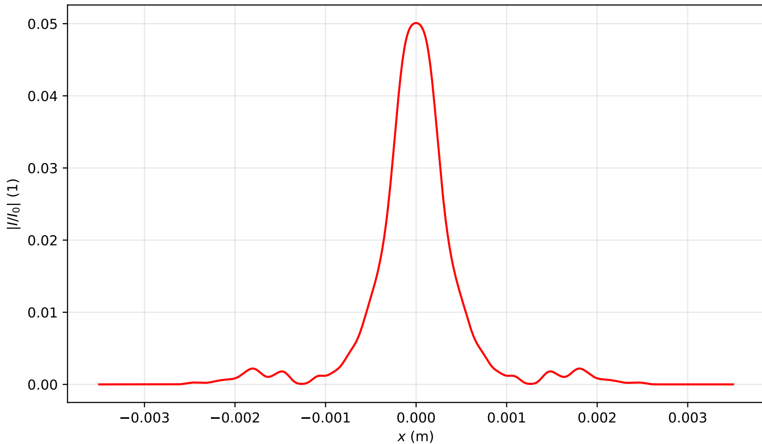
Intensity profile I(x, y = 0, z = 2.388)/I_0 , P_{in}=20.0\text{Pcr} , artificial time
