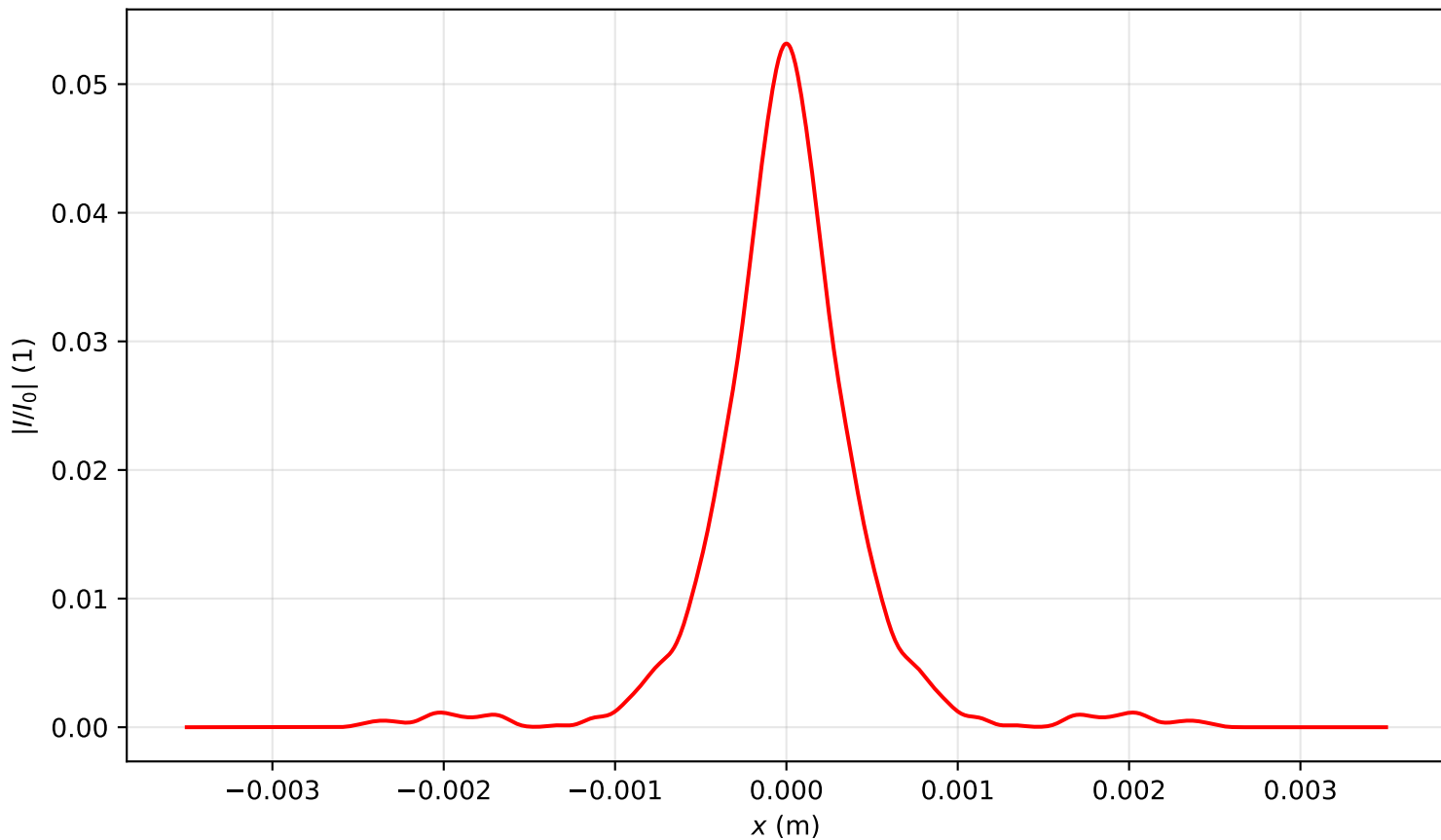
Intensity profile I(x, y = 0, z = 2.548)/I_0 , P_{in}=20.0\text{Pcr} , artificial time
