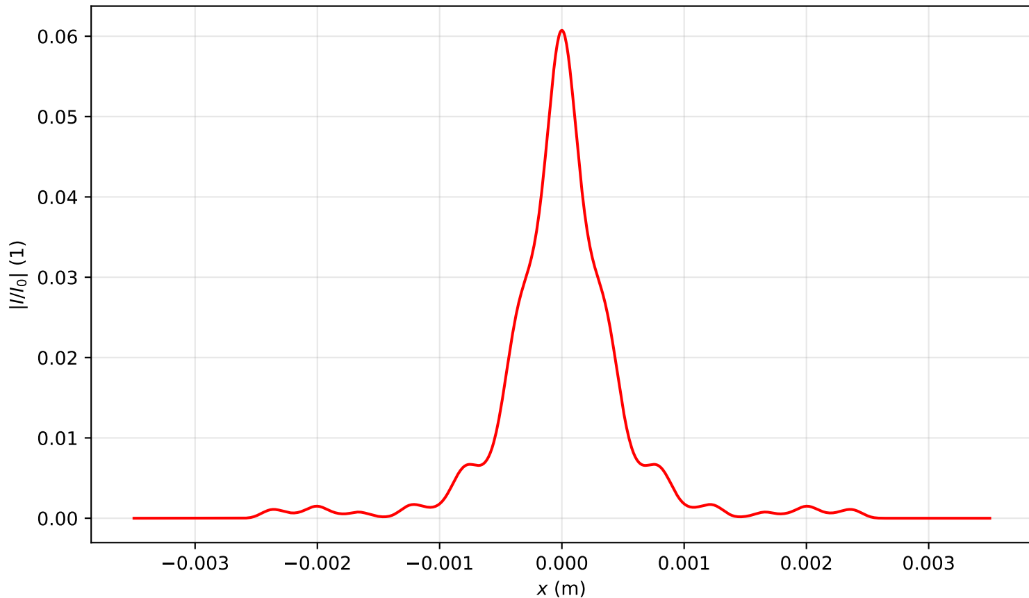
Intensity profile I(x, y = 0, z = 2.707)/I_0 , P_{in}=20.0P_{cr} , artificial time
