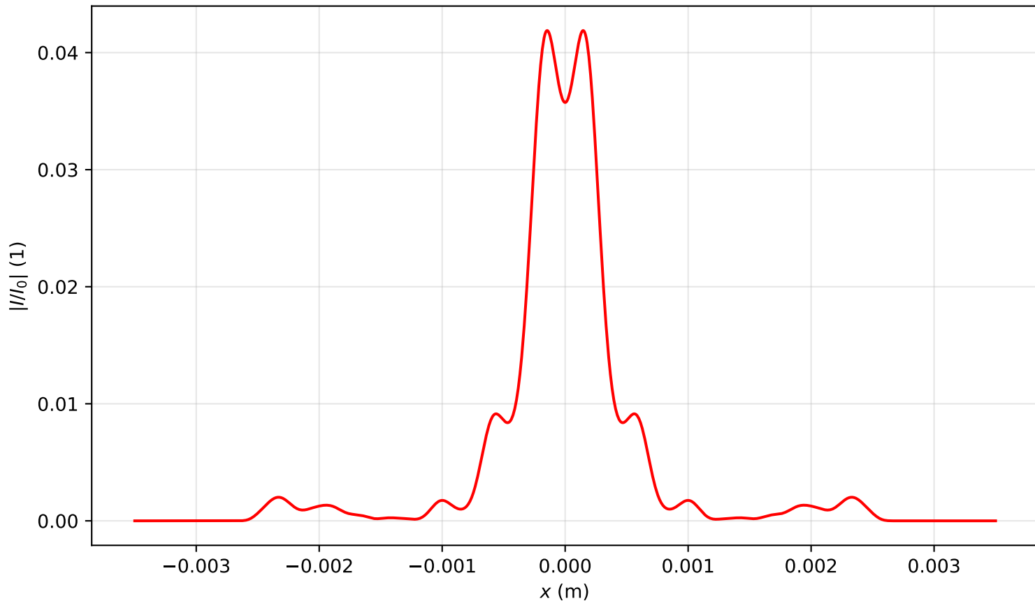
Intensity profile I(x, y = 0, z = 2.866)/I_0 , P_{in}=20.0\text{Pcr} , artificial time
