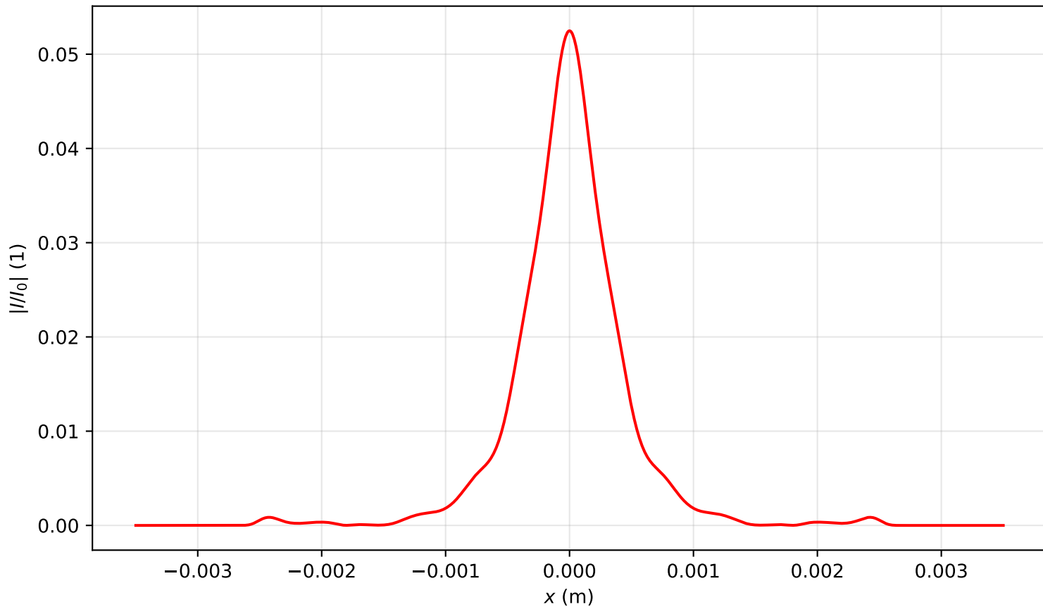
Intensity profile I(x, y = 0, z = 3.025)/I_0 , P_{in}=20.0\text{Pcr} , artificial time
