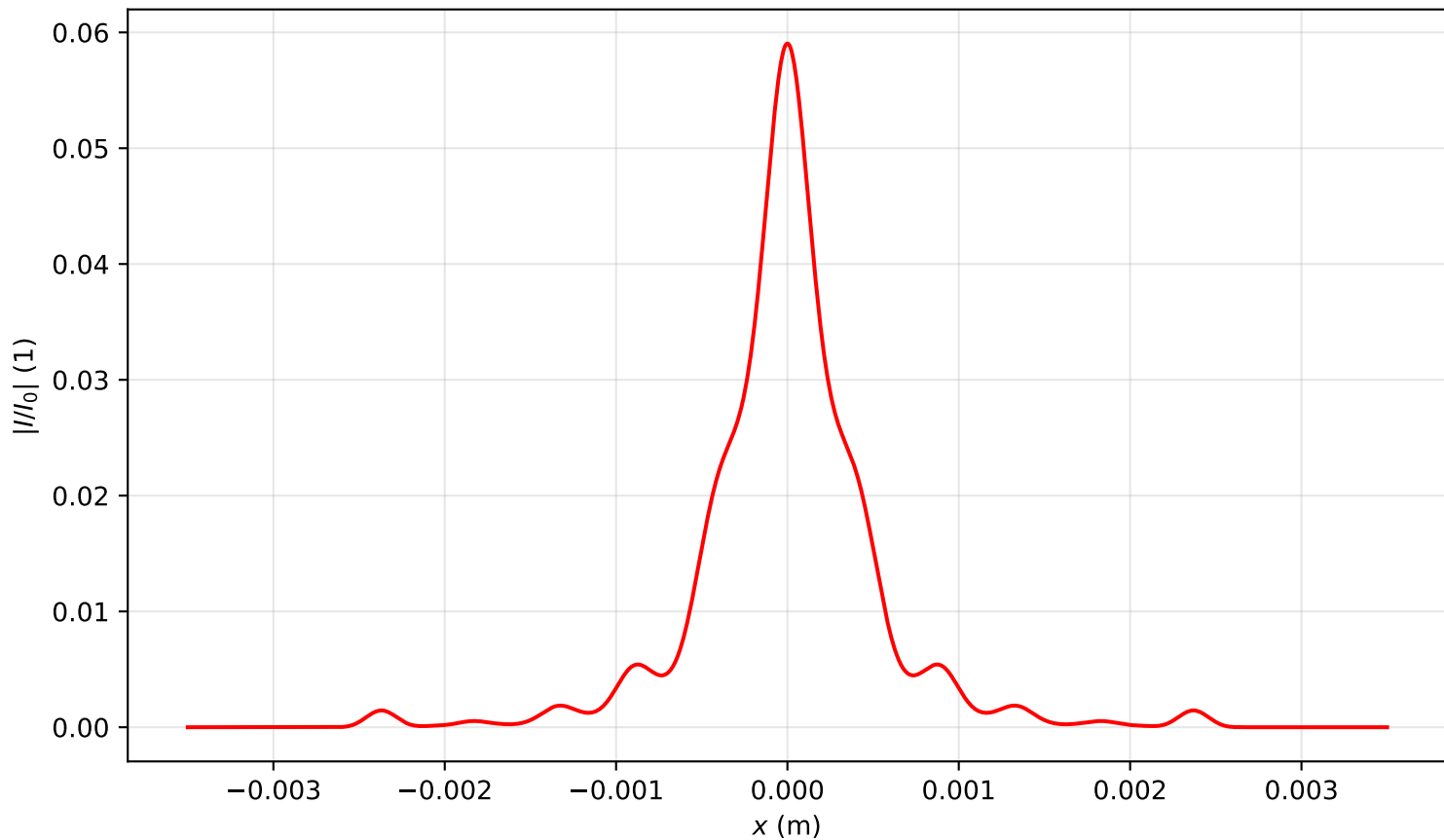
Intensity profile I(x, y = 0, z = 3.184)/I_0 , P_{in}=20.0\text{Pcr} , artificial time
