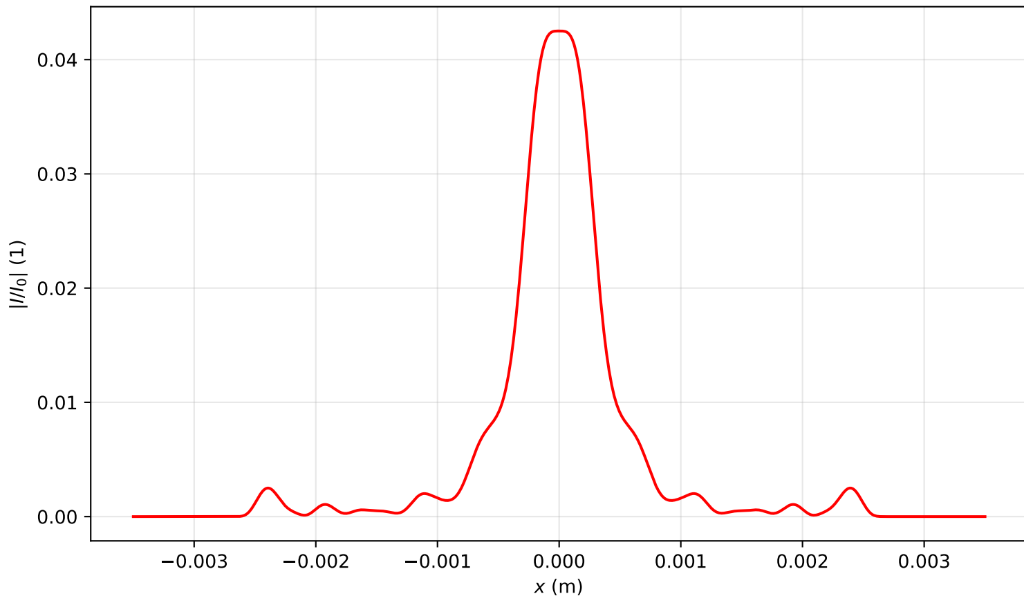
Intensity profile I(x, y = 0, z = 3.344)/I_0 , P_{in}=20.0P_{cr} , artificial time
