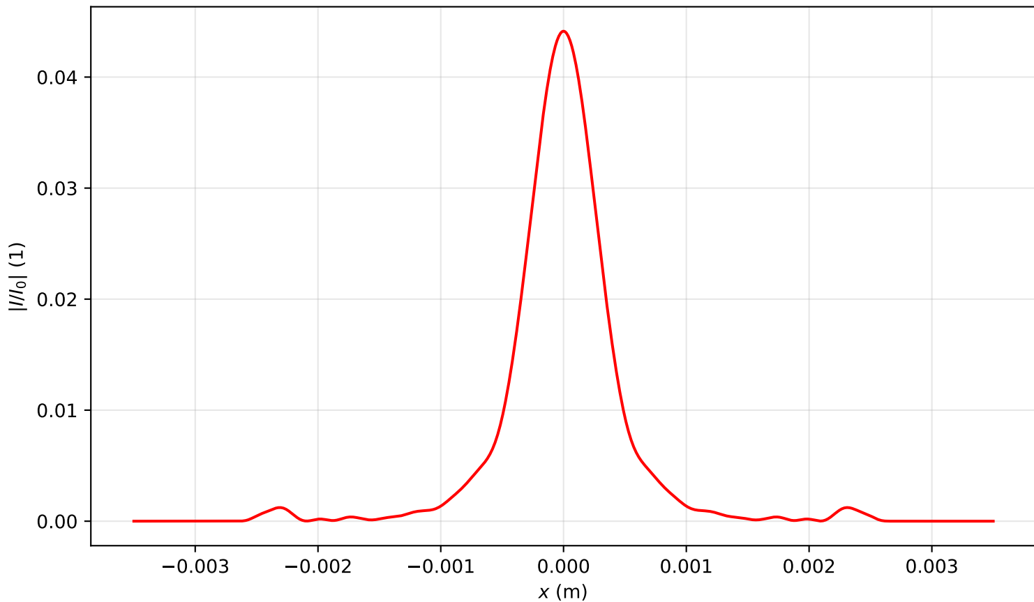
Intensity profile I(x, y = 0, z = 3.503)/I_0 , P_{in}=20.0\text{Pcr} , artificial time
