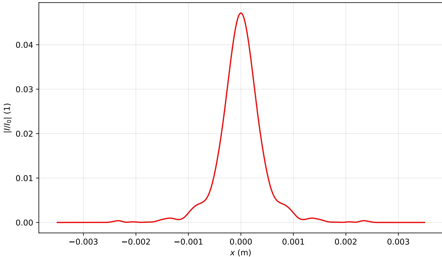
Intensity profile I(x, y = 0, z = 3.662)/I_0 , P_{in}=20.0P_{cr} , artificial time
