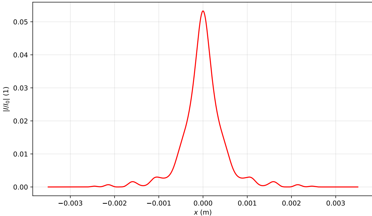
Intensity profile I(x, y = 0, z = 3.821)/I_0 , P_{in}=20.0\text{Pcr} , artificial time
