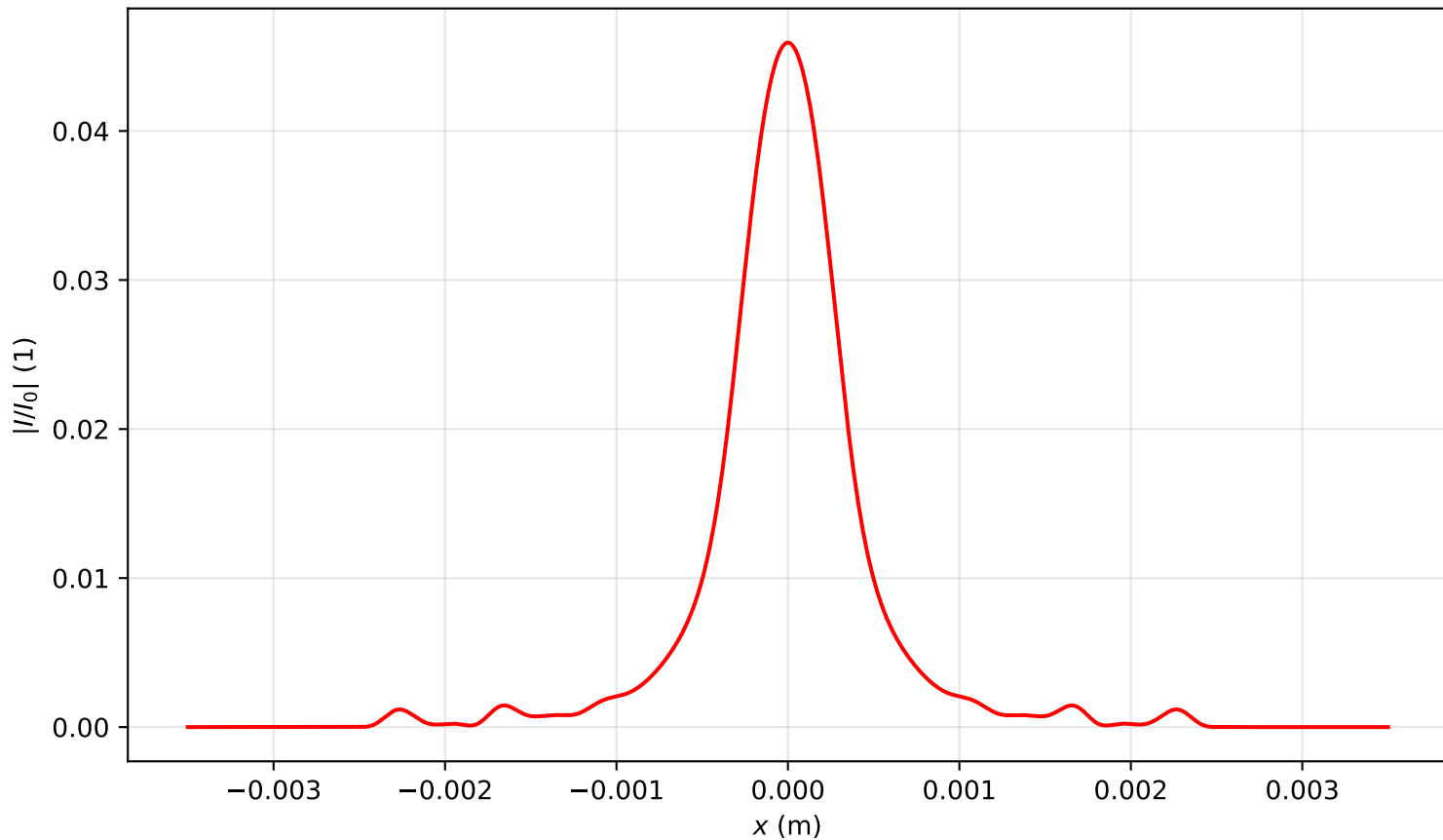
Intensity profile I(x, y = 0, z = 3.981)/I_0 , P_{in}=20.0\text{Pcr} , artificial time
