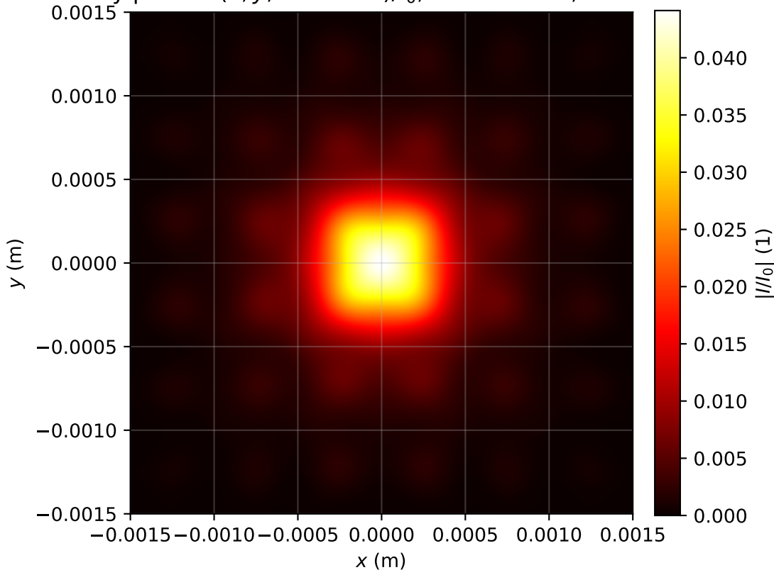
Intensity profile I(x, y, z = 3.503)/I_0 , P_{in}=20.0P_{cr} , artificial time
