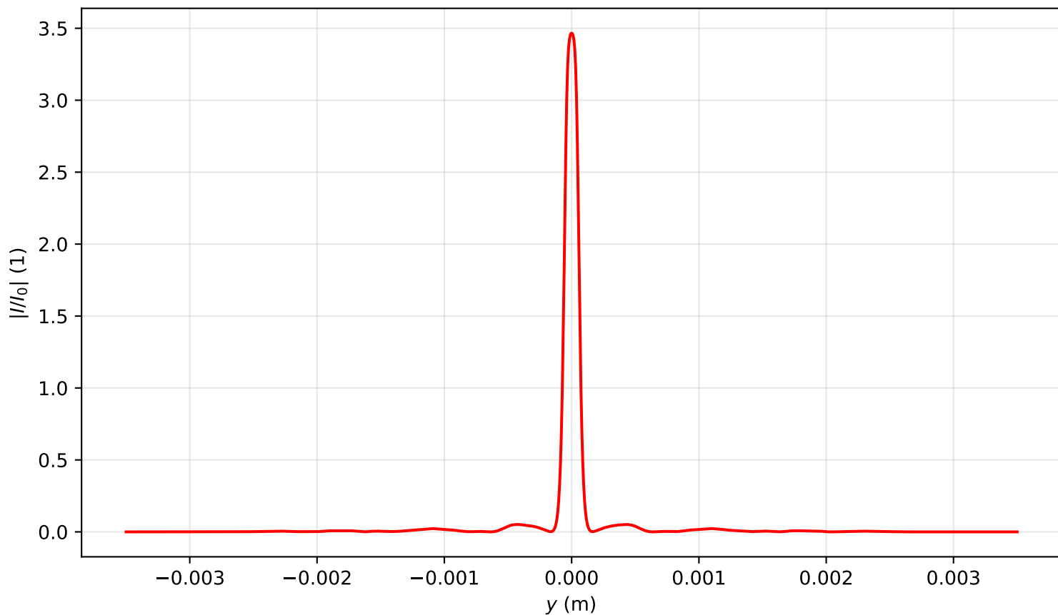
Intensity profile I(x=0, y, z=0.478)/I_0 , P_{in}=20.0P_{cr} , artificial time
