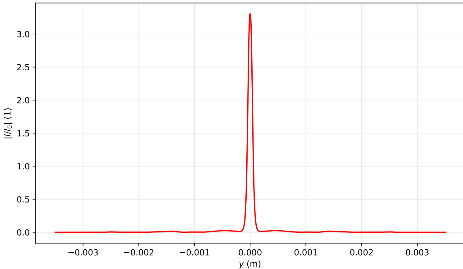
Intensity profile I(x=0, y, z=0.637)/I_0 , P_{in}=20.0P_{cr} , artificial time
