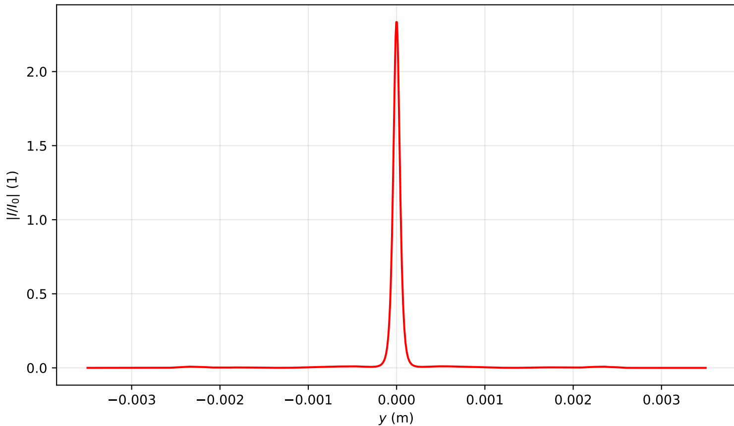
Intensity profile I(x=0, y, z=0.955)/I_0 , P_{in}=20.0P_{cr} , artificial time
