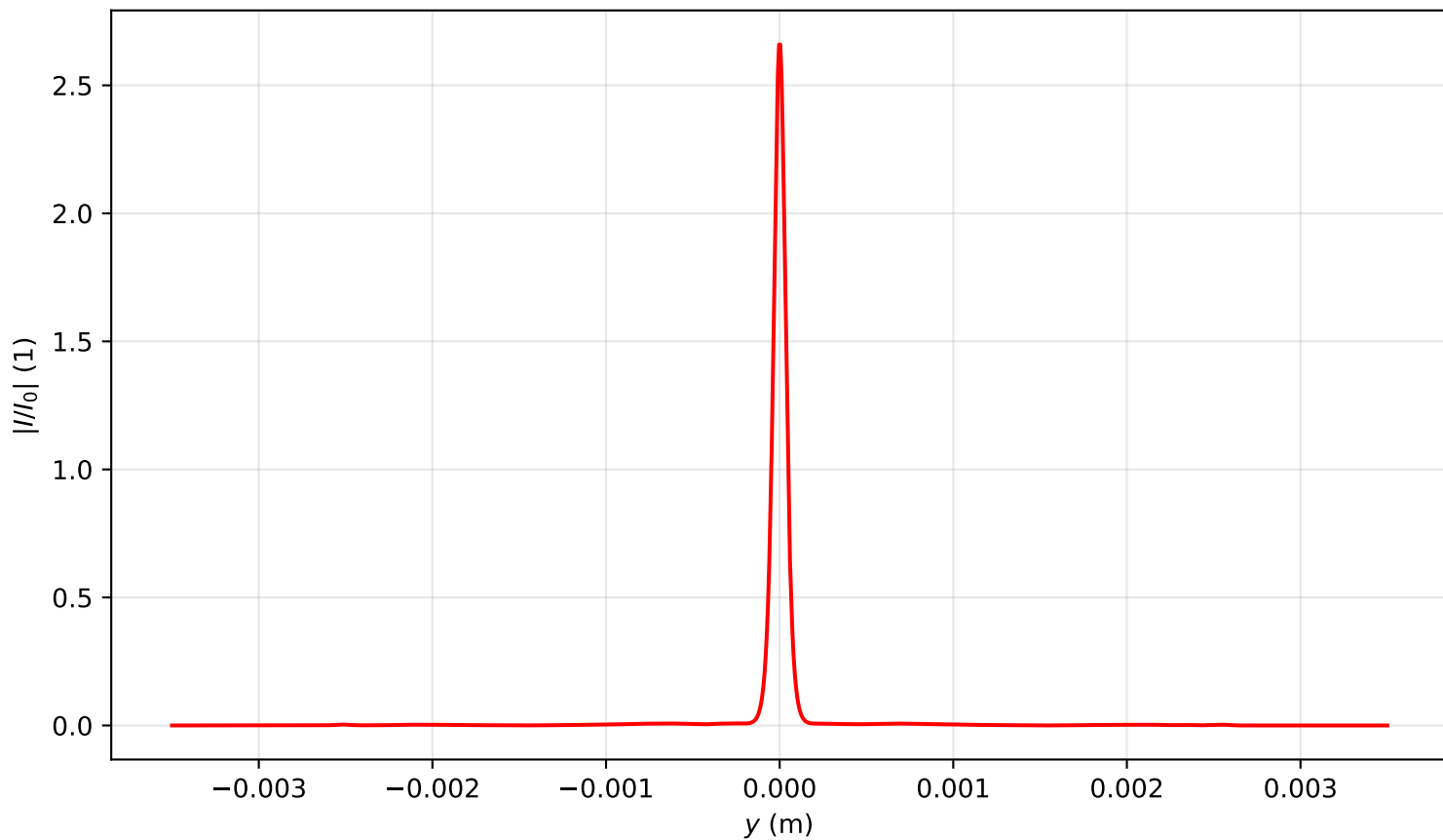
Intensity profile I(x=0, y, z=1.115)/I_0 , P_{in}=20.0P_{cr} , artificial time
