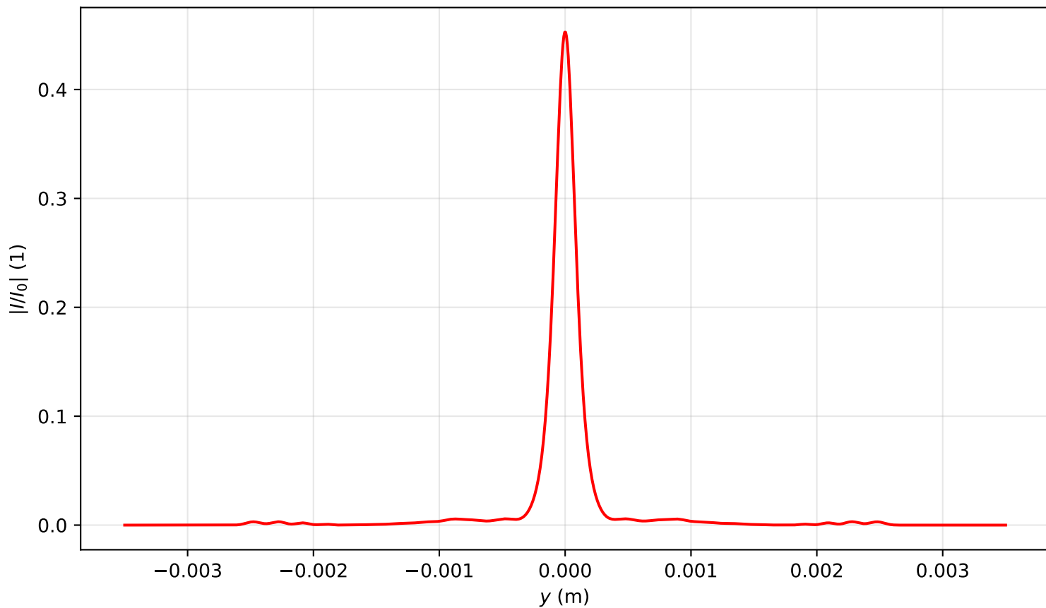
Intensity profile I(x=0, y, z=1.274)/I_0 , P_{in}=20.0P_{cr} , artificial time
