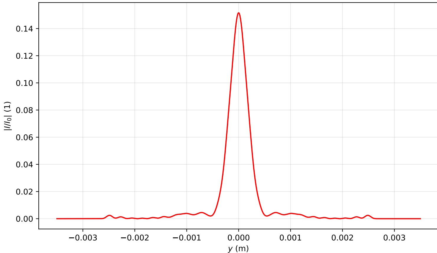
Intensity profile I(x=0, y, z=1.433)/I_0 , P_{in}=20.0\text{Pcr} , artificial time
