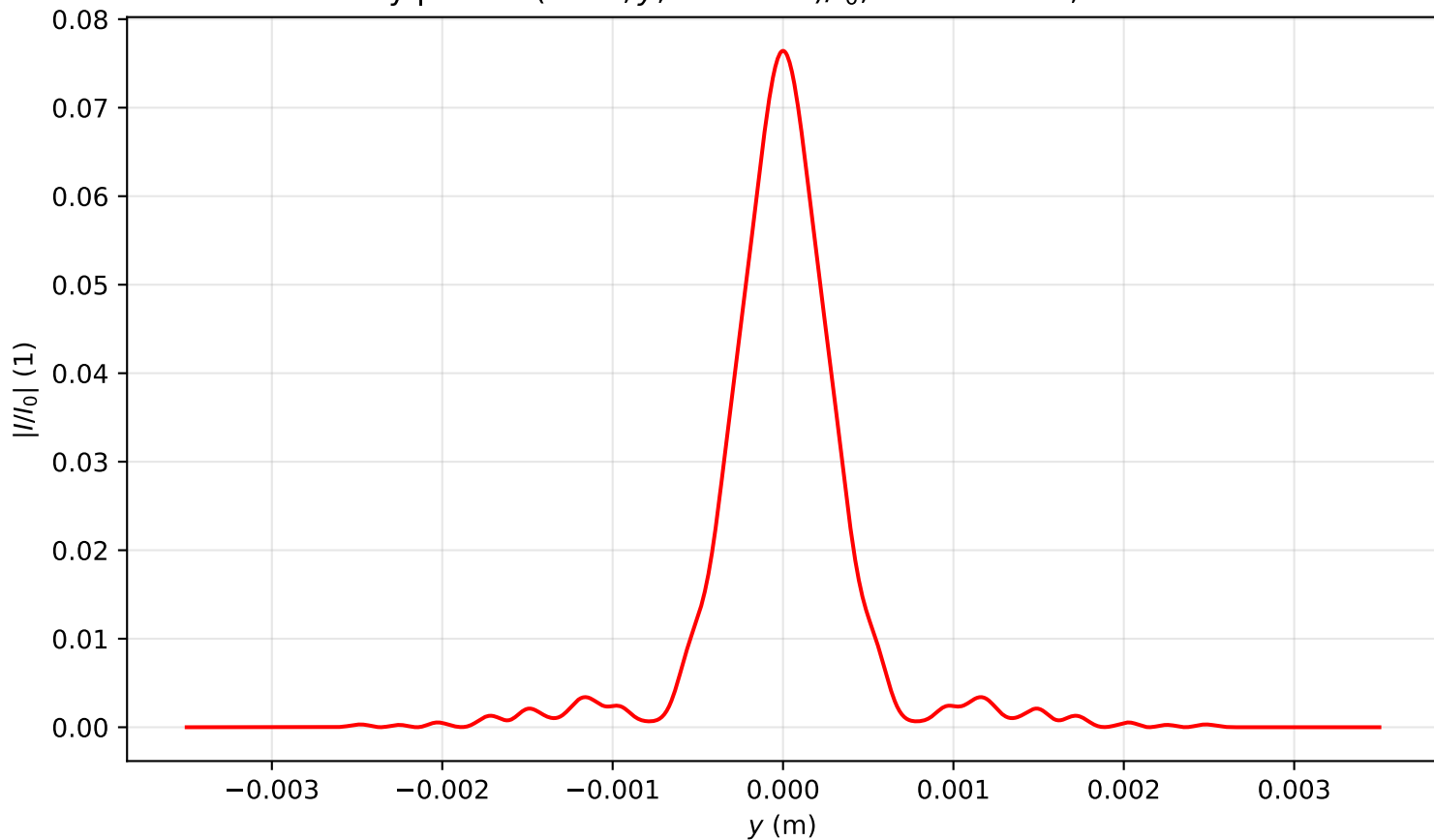
Intensity profile I(x=0, y, z=1.751)/I_0 , P_{in}=20.0P_{cr} , artificial time
