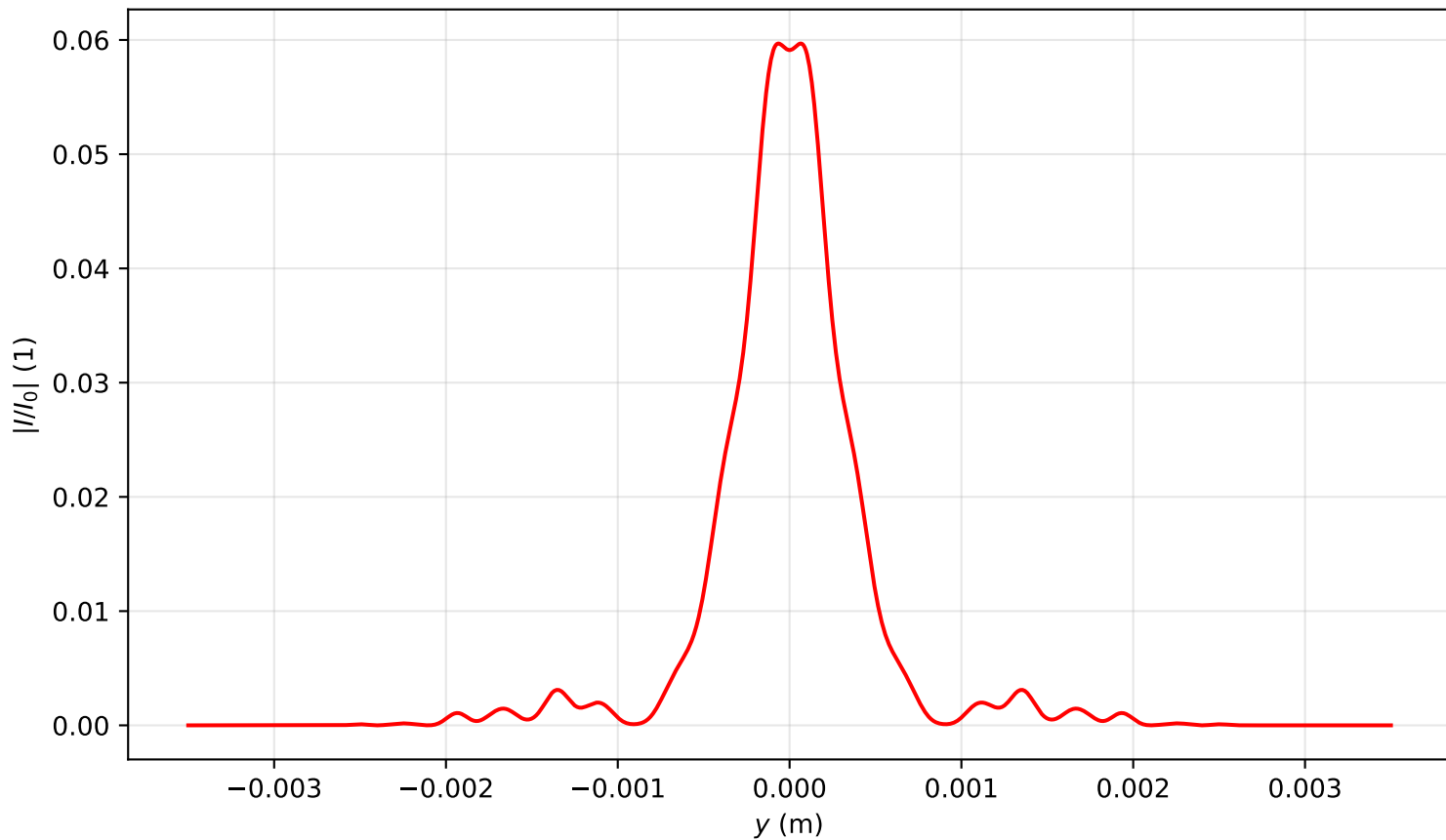
Intensity profile I(x=0, y, z=1.911)/I_0 , P_{in}=20.0\text{Pcr} , artificial time
