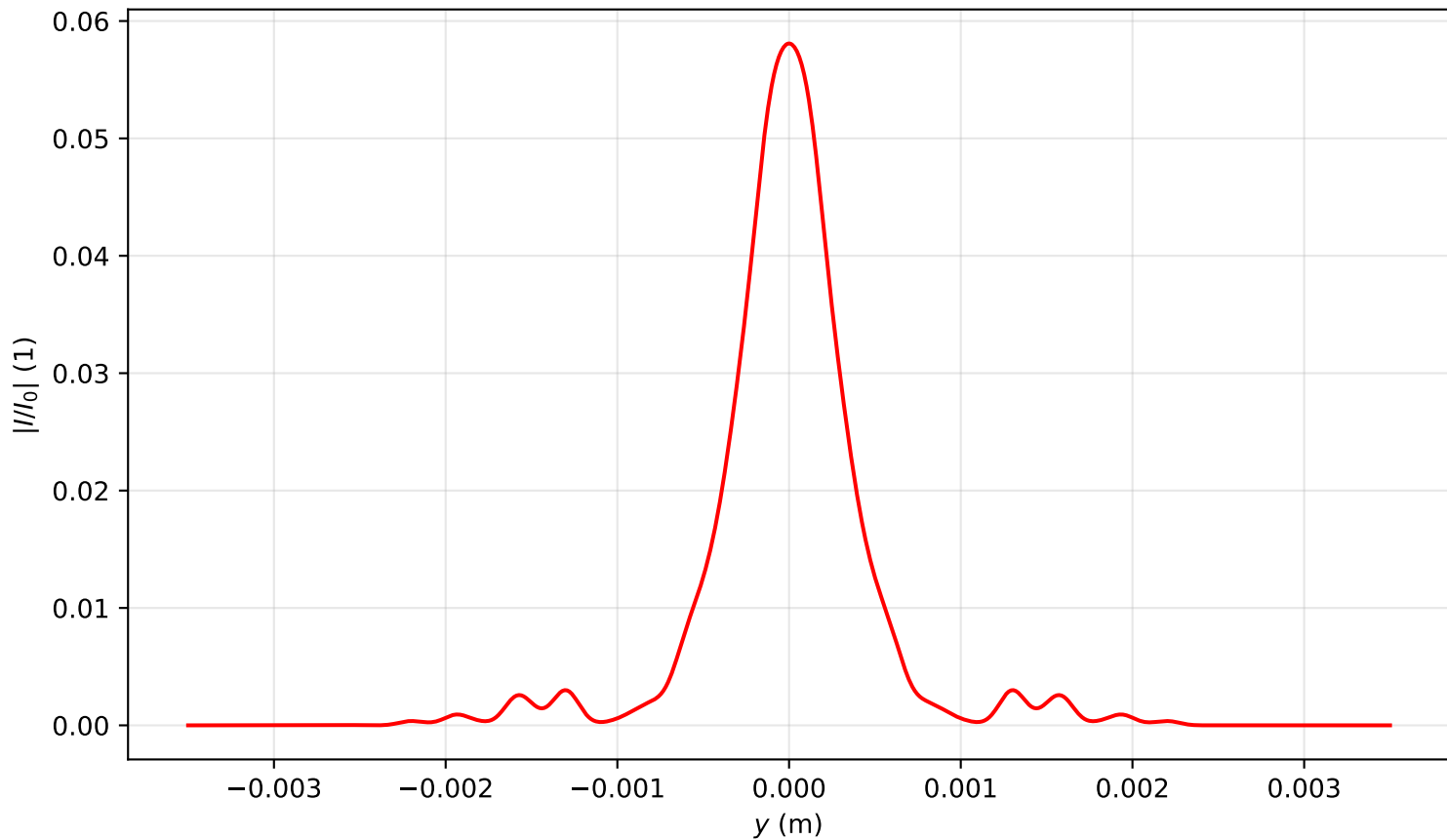
Intensity profile I(x = 0, y, z = 2.070)/I_0 , P_{in}=20.0P_{cr} , artificial time
