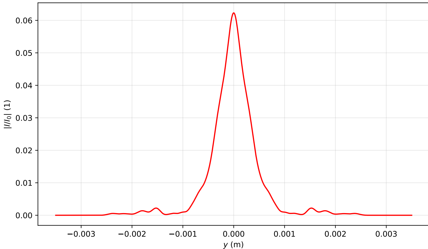
Intensity profile I(x = 0, y, z = 2.229)/I_0 , P_{in}=20.0P_{cr} , artificial time
