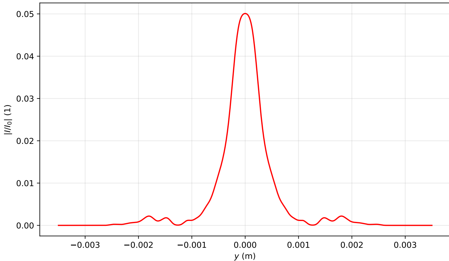
Intensity profile I(x=0, y, z=2.388)/I_0 , P_{in}=20.0P_{cr} , artificial time
