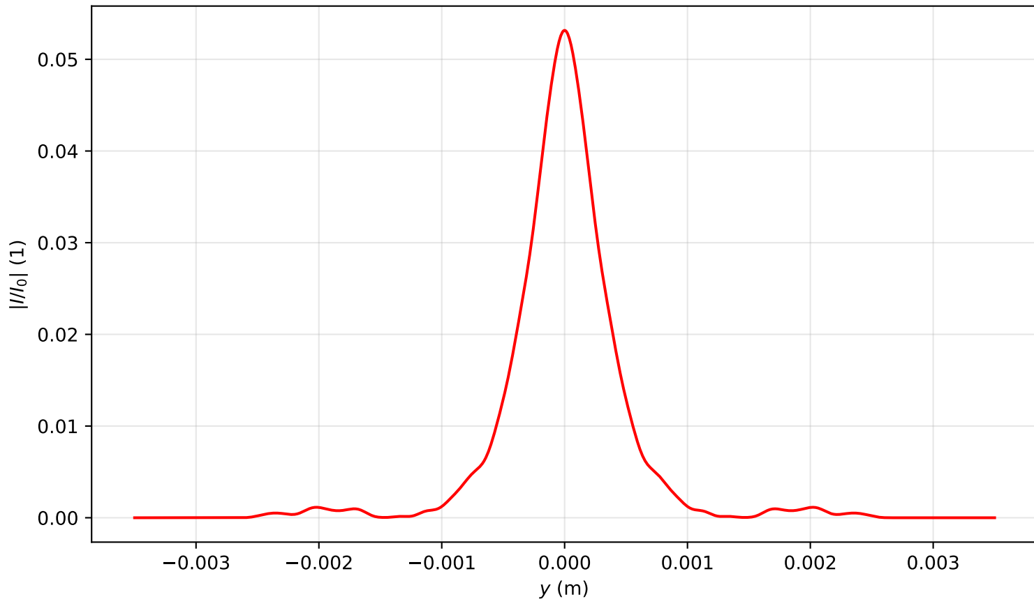
Intensity profile I(x = 0, y, z = 2.548)/I_0 , P_{in}=20.0P_{cr} , artificial time
