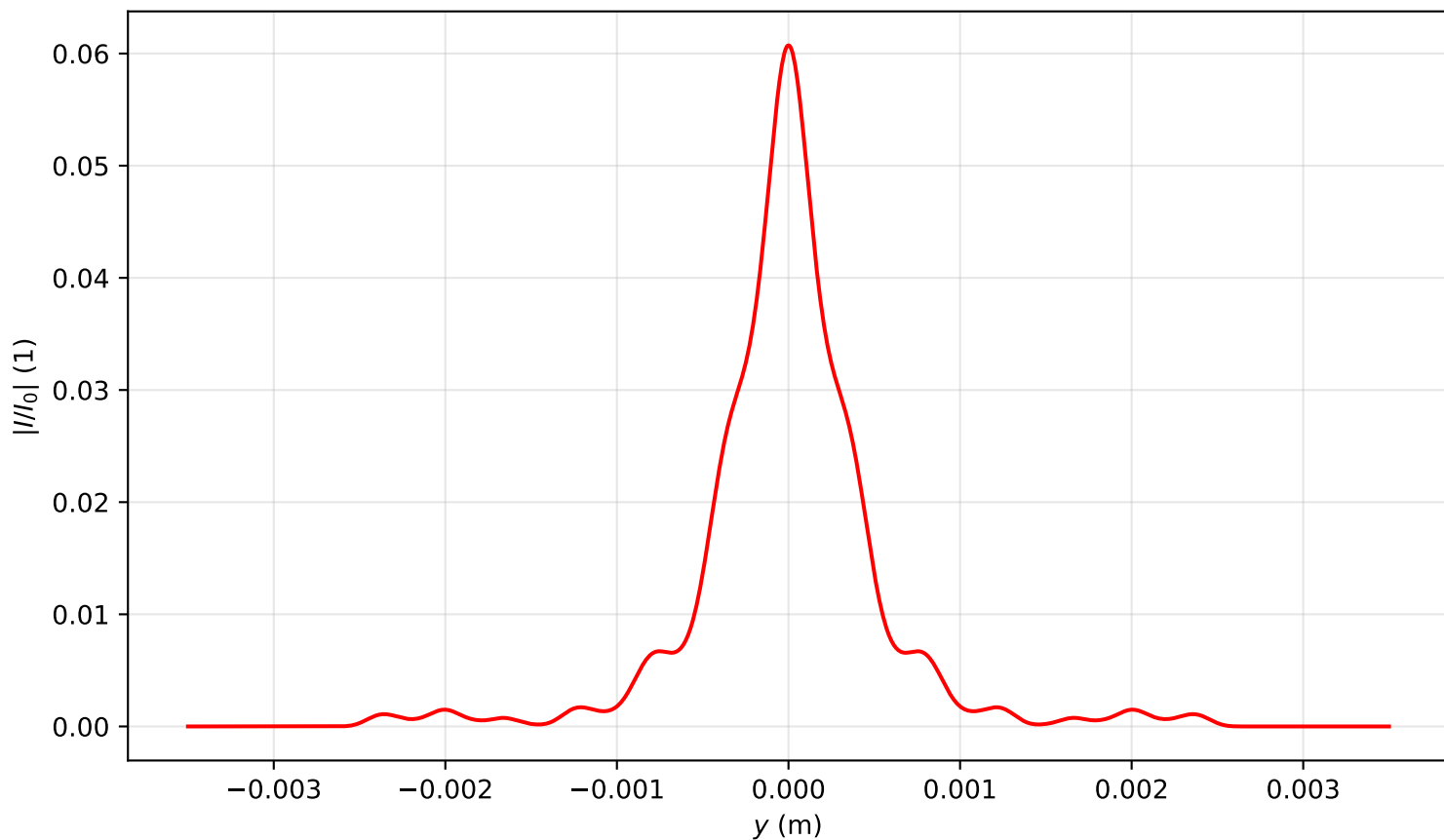
Intensity profile I(x = 0, y, z = 2.707)/I_0 , P_{in}=20.0P_{cr} , artificial time
