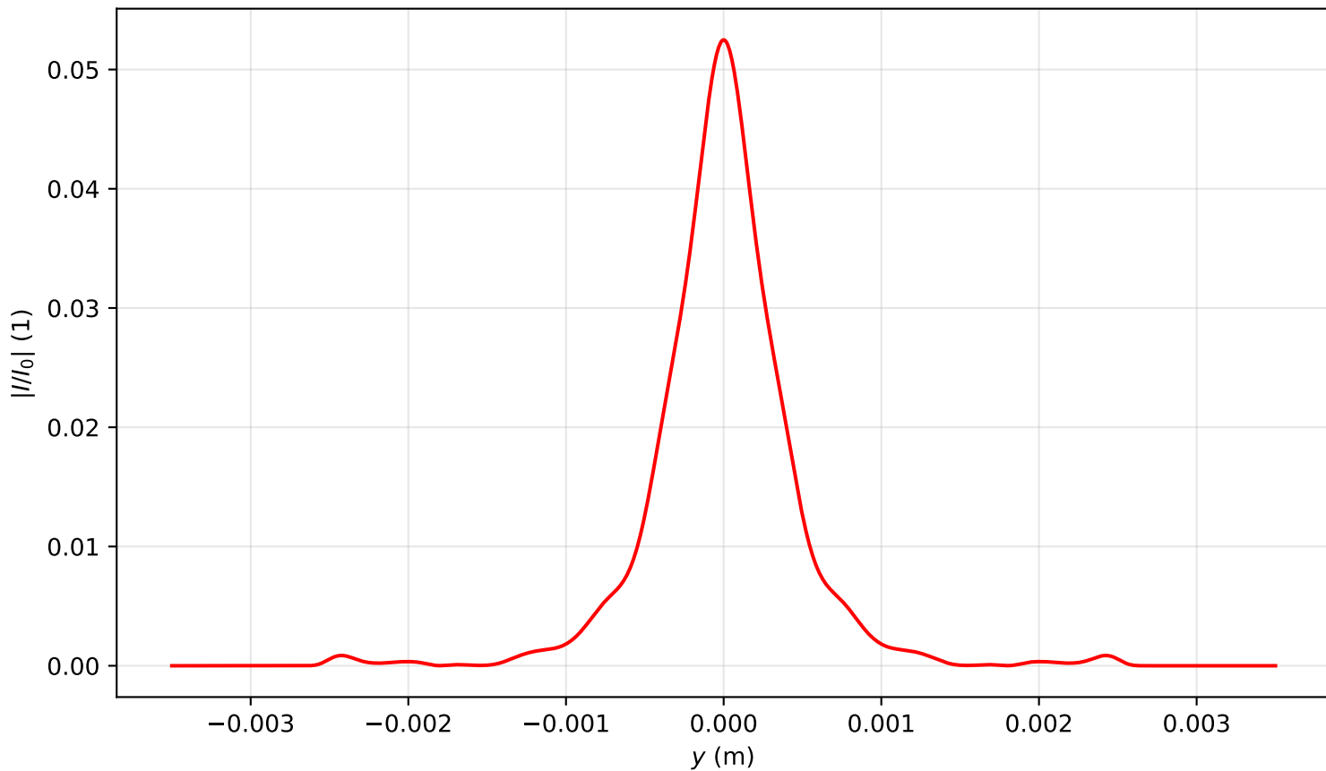
Intensity profile I(x = 0, y, z = 3.025)/I_0 , P_{in}=20.0\text{Pcr} , artificial time
