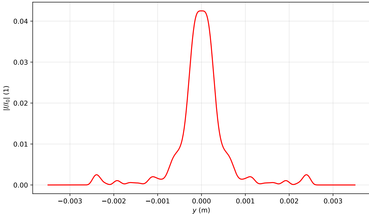
Intensity profile I(x = 0, y, z = 3.344)/I_0 , P_{in}=20.0P_{cr} , artificial time
